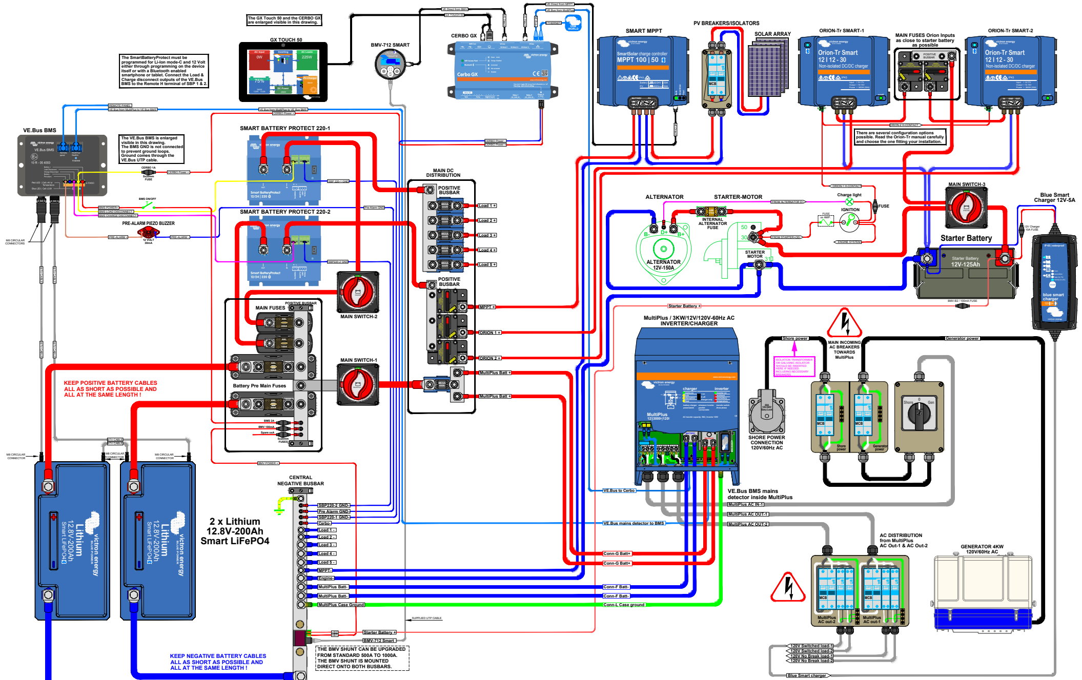
Drawing BJE-276C
